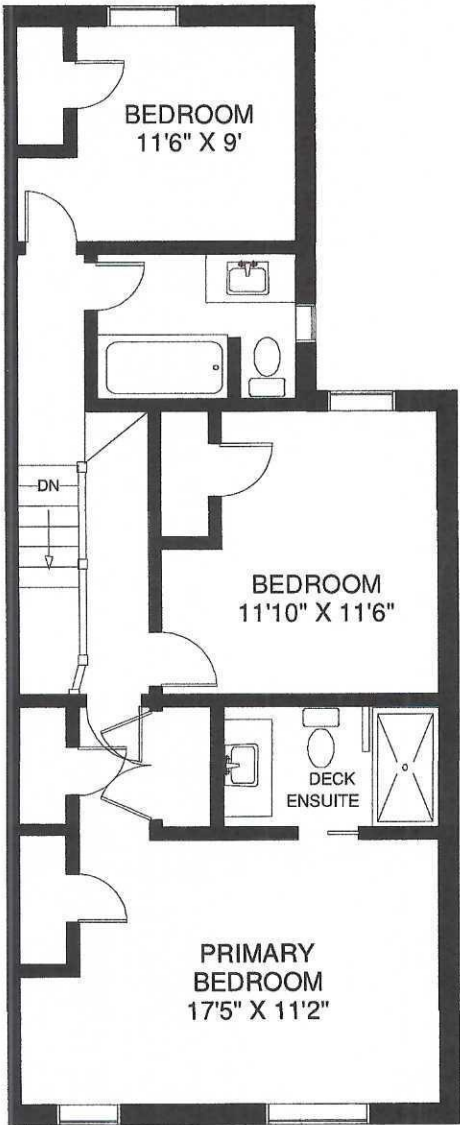
SECOND FLOOR APPROXIMATELY 775 SQ FT
